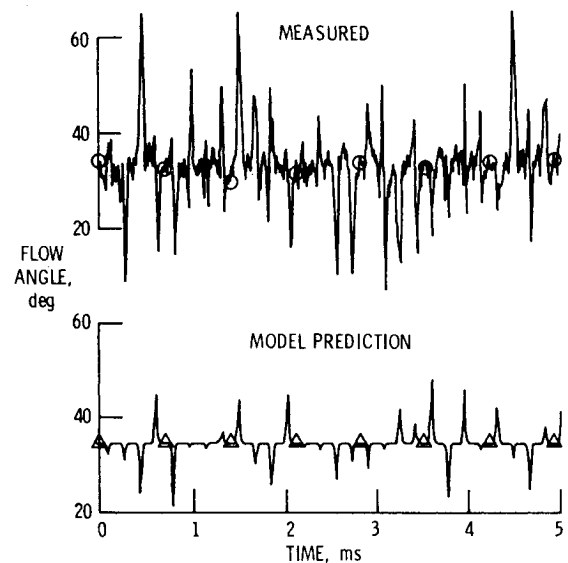
Fig. 12 Comparison of rotor exit relative flow measured with ellipse probe to prediction by wake model.
