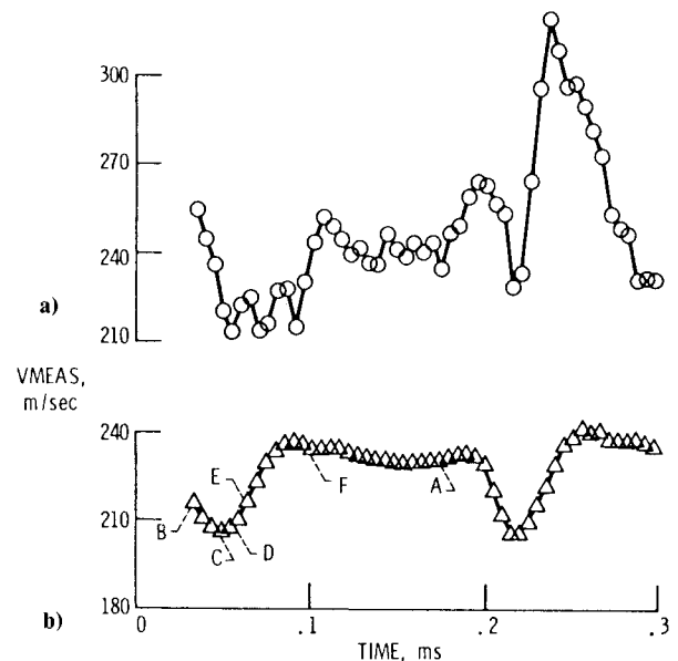
Fig. 5 Velocity component of probe measurement corresponding to LA measurement in Fig. 2: a) instantaneous, b) 90 rotor revolutions ensemble average.
