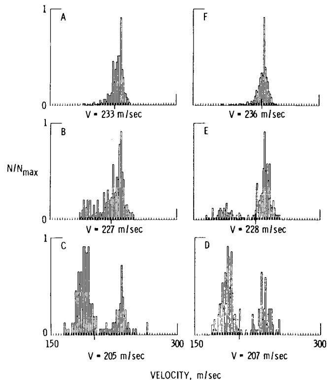
Fig. 3 Probability density distributions of velocity at points A–F in Fig. 2.
