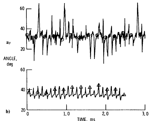
Fig. 4 a) Instantaneous relative flow angle at 140% chord measured with the ellipse probe; b) as in part a, but rotor ensemble-averaged over 90 rotor revolutions.
