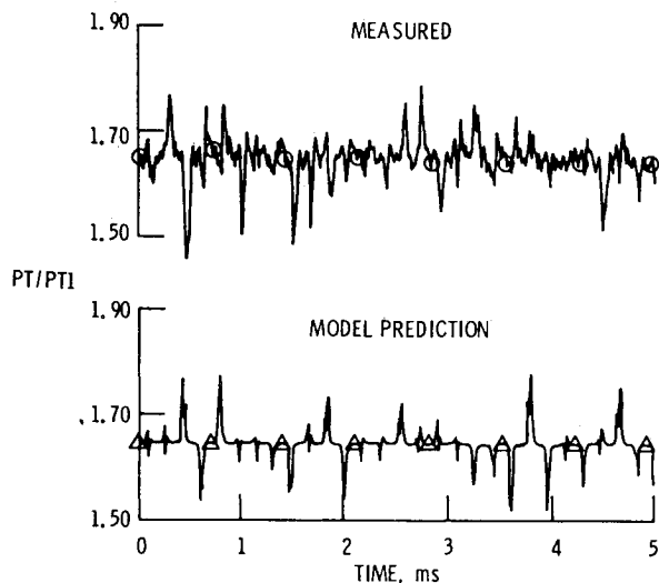
Fig. 13 Comparison of rotor total pressure ratio measured with probe to prediction by wake model.
