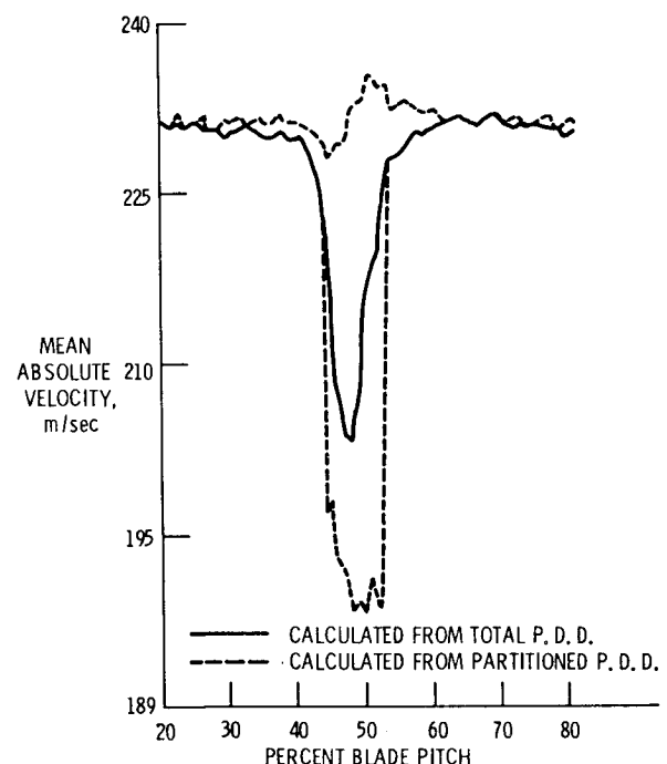
Fig. 8 Distribution of mean absolute velocity as measured by LA, including effect of partitioning probability density distribution.
