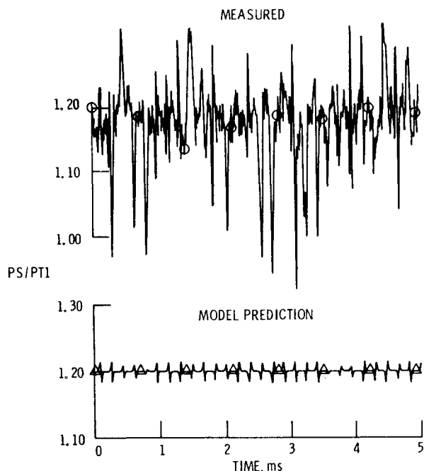
Fig. 14 Comparison of rotor exit static to upstream total pressure ratio as measured by probe to wake model prediction.
