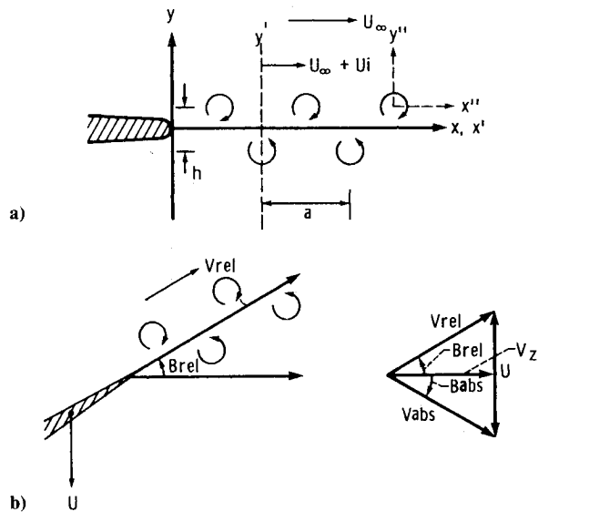
Fig. 9 Geometry and nomenclature used in blade wake vortex model.
