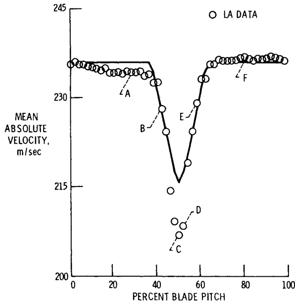
Fig. 10 Comparison of LA data from Fig. 2 with wake model fit.
