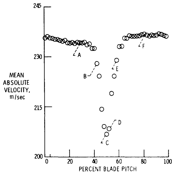
Fig. 2 Mean absolute velocity distribution measured by the LA at 60% span, 140% chord in a plane 42 deg from the axial direction.
