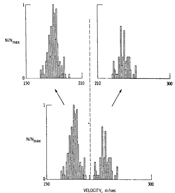
Fig. 7 Partitioning of bimodal probability density distribution obtained in the wake.
