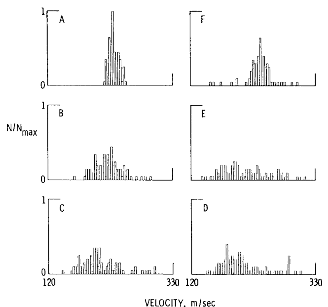
Fig. 6 Probability density distribution of component of probe measurement shown in Fig. 5 at corresponding points.
